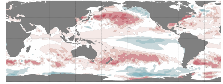
Figure 1: Feb - Apr 2022 Sea Surface Temperature (SST) Anomaly Forecast
