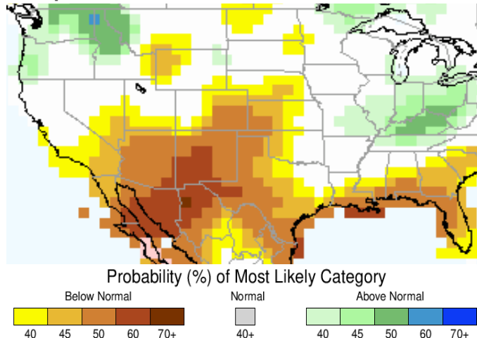
Figure 7A: Three-Month (Feb-Apr) Forecast for Precipitation
