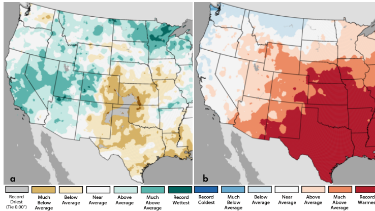
Figure 1: Dec 2021 Precipitation (a) & Temperature Ranks (b)
