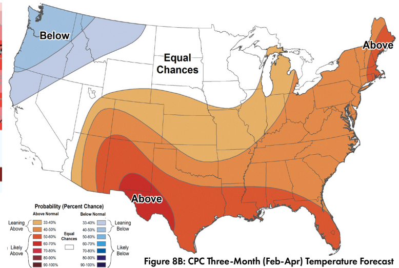
Figure 8B: CPC Three-Month (Feb-Apr) Temperature Forecast
