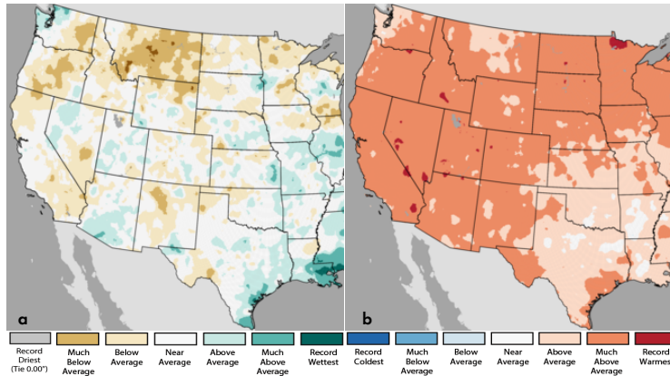
Figure 2: Jan-Dec 2021 Precipitation (a) & Temperature Ranks (b)
