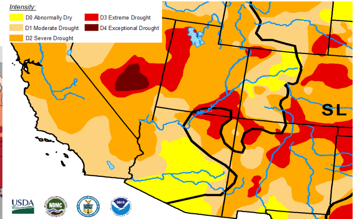
Figure 4: US Drought Monitor - Jan 11, 2022
