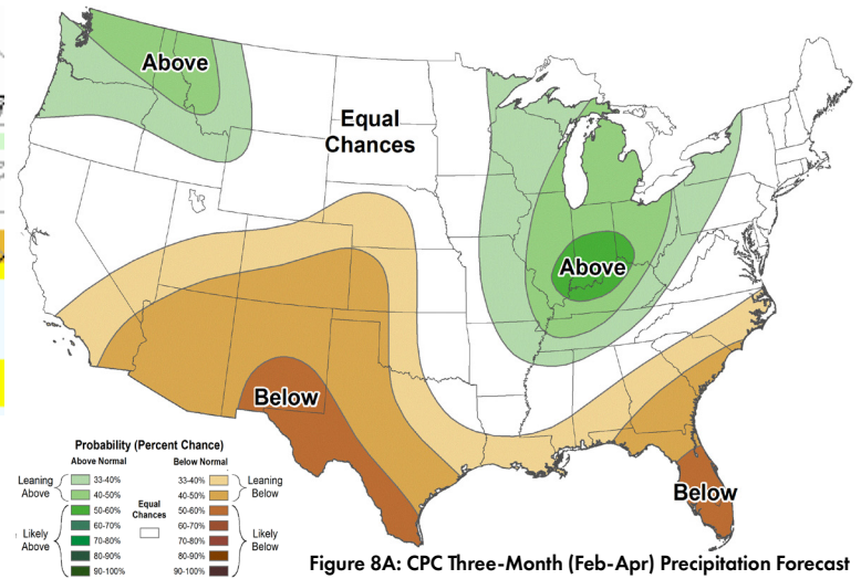
Figure 8A: CPC Three-Month (Feb-Apr) Precipitation Forecast
