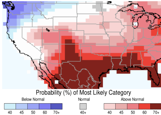
Figure 7B: Three-Month (Feb-Apr) Forecast for Temperature
